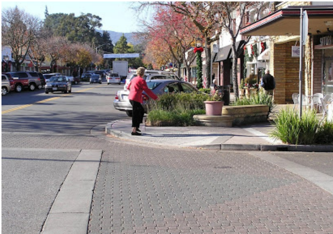
Bulb-out corners improve crossings for pedestrians
